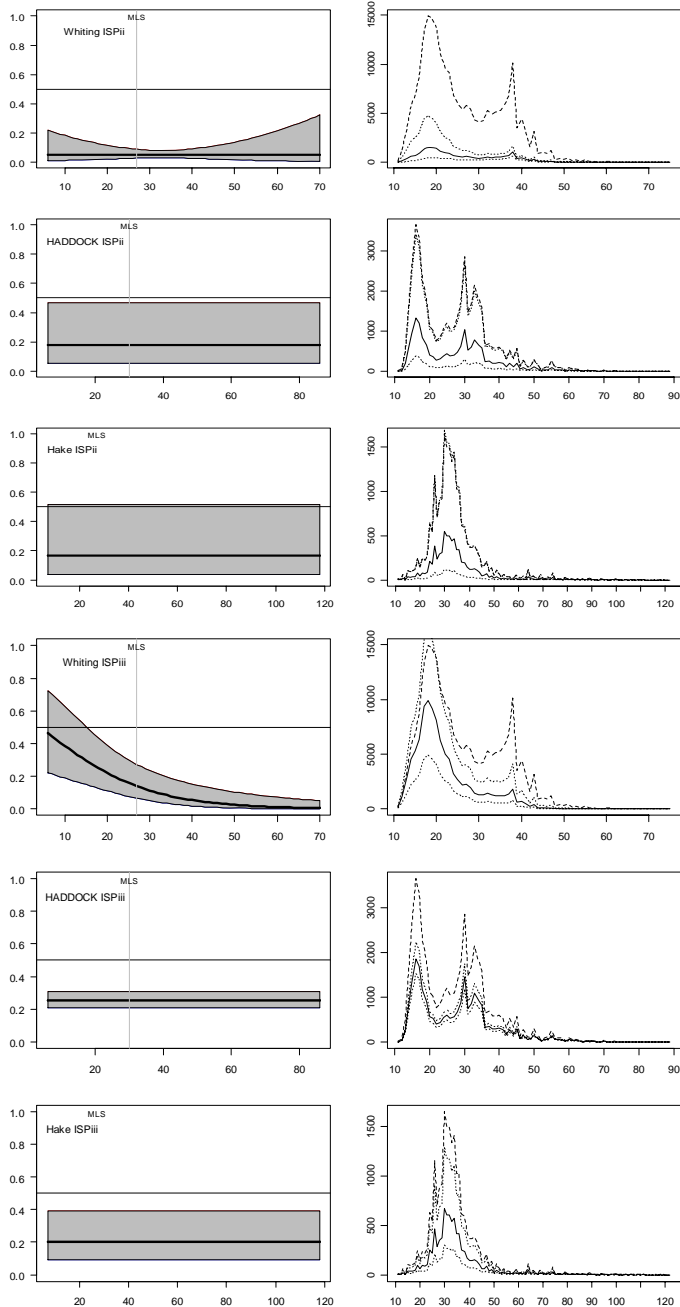
Figure 28. Left plots show the modelled proportion of the number of whiting, haddock and hake at length caught in trawls with an inclined separator panel (version 2) in the Irish Sea relative to the total in both a conventional trawl and a trawl with a modification (i.e. 0.5 indicates an equal number caught in both trawls). Two trials were conducted and were analysed separately. Grey shaded area is area of significance around the modelled fit. MLS = minimum landing size. Right plots give catch length frequency from the sampled trips (dashed line) and the predicted change in catch length frequency with the use of a gear modification (solid line, with area of significance as dotted line).
