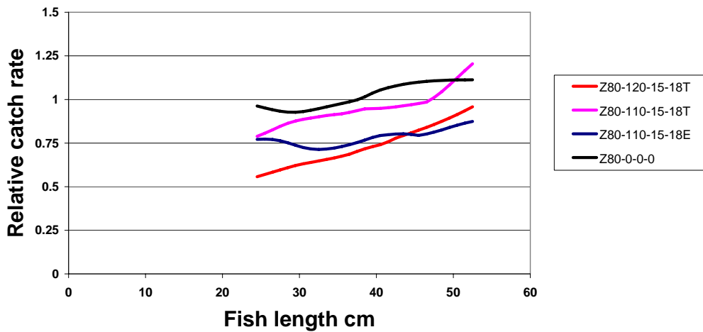
Figure 19 Hake selectivity with a 110 or 120mm, 3m long square mesh panel inserted in the taper or extension of the trawl.
