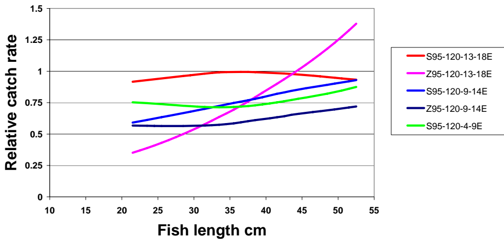
Figure 21. Nephrops selectivity with a 120mm, 5m long square mesh panel inserted in various positions of the extension.
