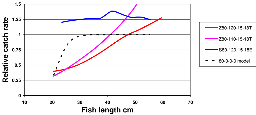
Figure 16. Cod selectivity with a 110 or 120mm, 3m long square mesh panel inserted in the taper or extension of the trawl.
