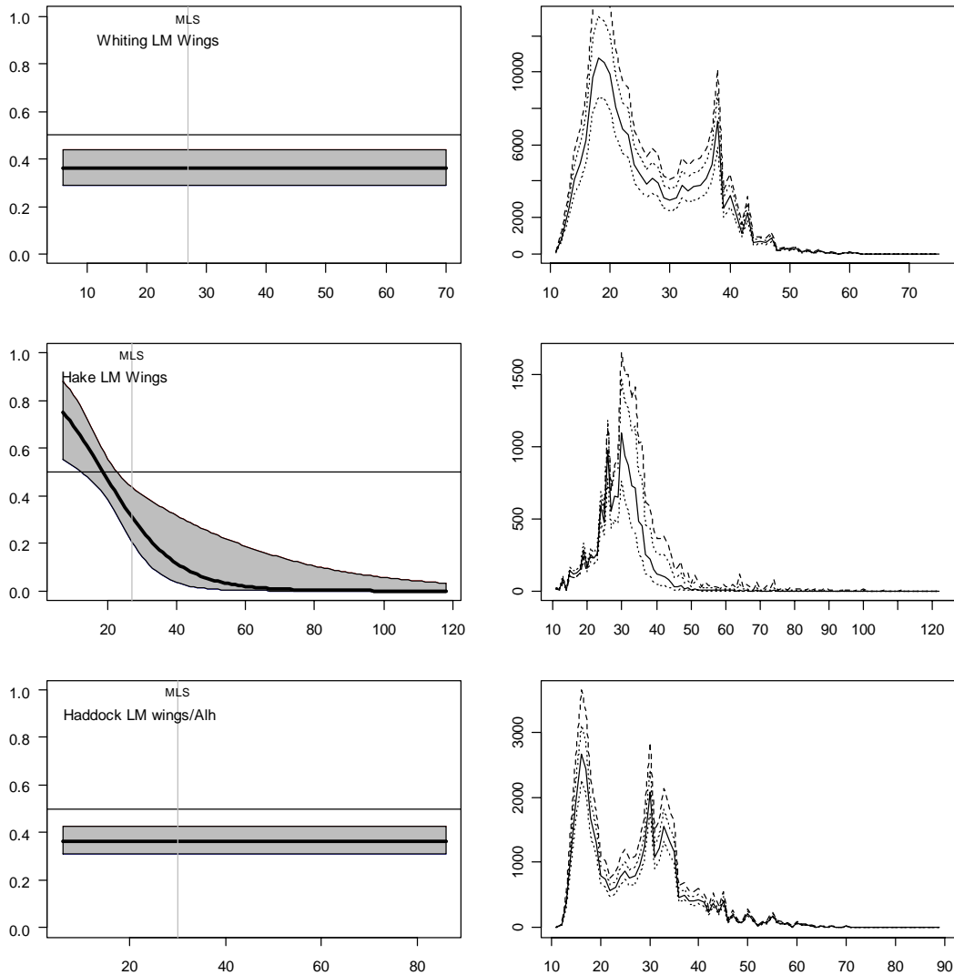
Figure 29. Left plots show the modelled proportion of the number of whiting, hake and haddock at length caught in trawls with large mesh wings in the Irish Sea relative to the total in both a conventional trawl and a trawl with a modification (i.e. 0.5 indicates an equal number caught in both trawls). Two trials were conducted and were analysed separately. Grey shaded area is area of significance around the modelled fit. MLS = minimum landing size. Right plots give catch length frequency from the sampled trips (dashed line) and the predicted change in catch length frequency with the use of a gear modification (solid line, with area of significance as dotted line).
