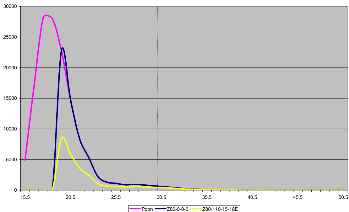
Figure 22 Comparison between a standard and more selective gear when fished on a haddock population comprising mainly of small fish. The vertical line is the MLS.
