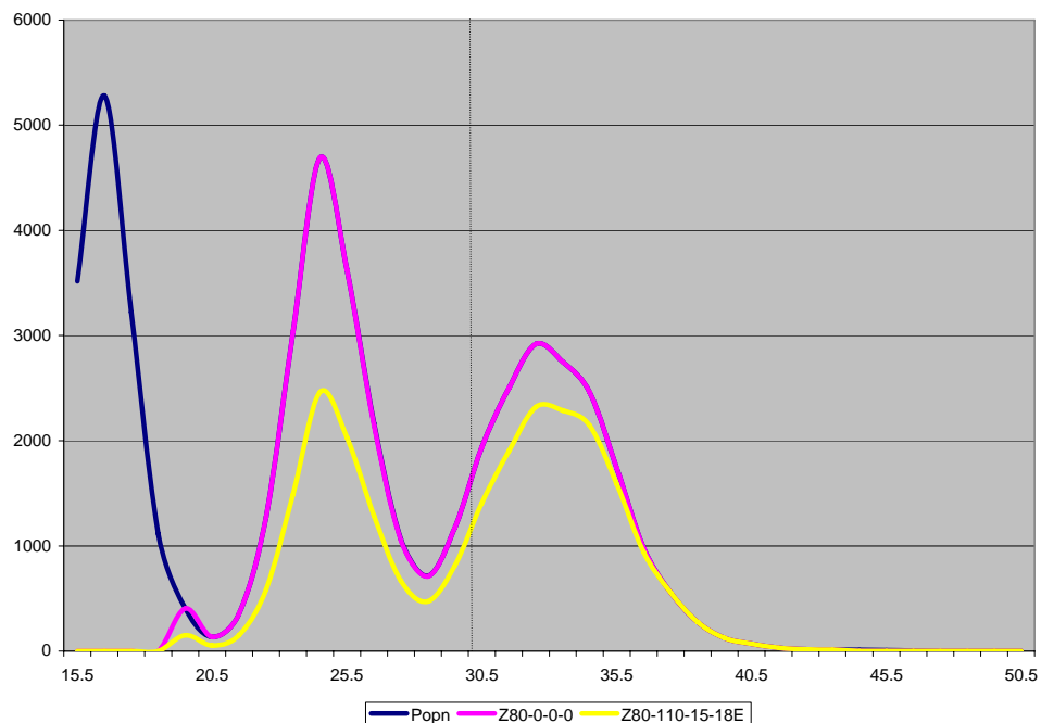
Figure 23 Comparison between a standard and more selective gear when fished on a haddock population with a broad length spectrum. The vertical line is the MLS.
