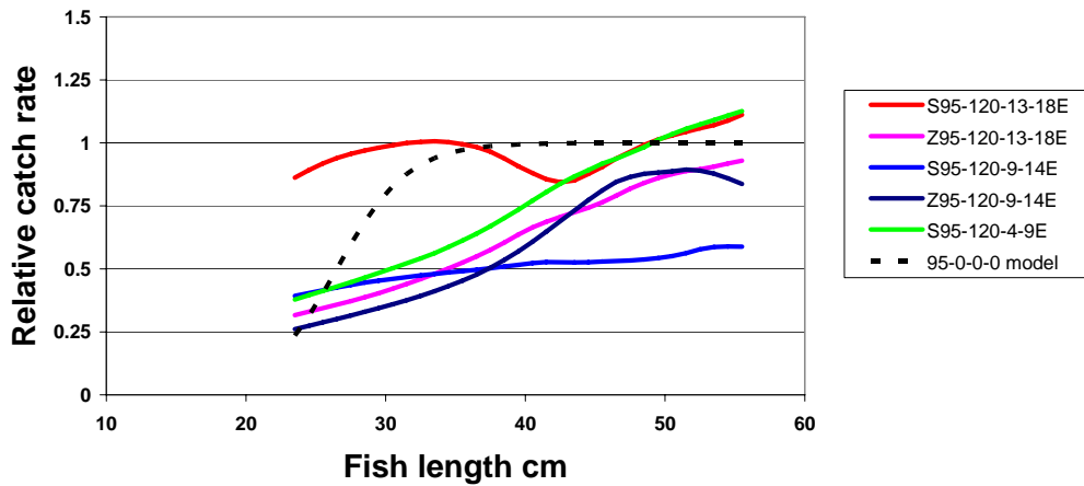
Figure 15 Cod selectivity with a 120mm, 5m long square mesh panel inserted in various positions of the extension.
