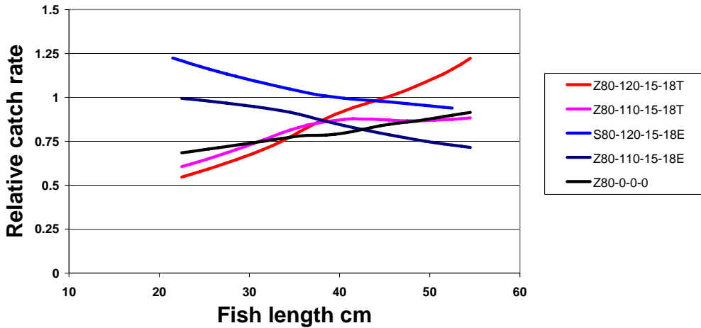
Figure 20. Nephrops selectivity with a 110 or 120mm, 3m long square mesh panel inserted in the taper or extension of the trawl.
