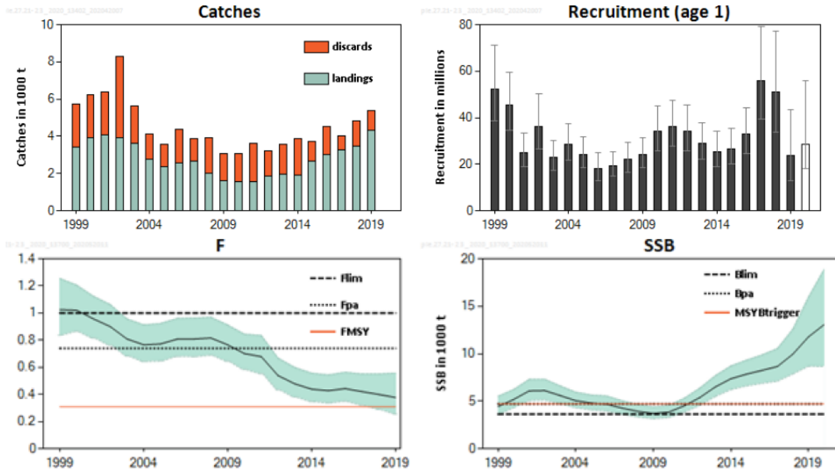
Figure 6: Baltic Plaice stock in subdivision 21-23. Summary of the stock assessment. Recruitment, F and SSB show confidence intervals (95%) in the plot. BMS landings (fish below the minimum conservation reference size [MCRS]) have been included since 2017. Figure taken from ICES 2020d.
