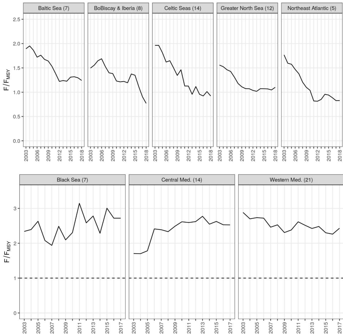
Figure 60: Trend in F/F_{MSY} by ecoregion in FAO 27. The number of stocks in each ecoregion is shown between parentheses (extracted from STECF-20-01 Monitoring the performance of the CFP). Due to the low number of stocks available for the Eastern Mediterranean, the indicator is not shown.
