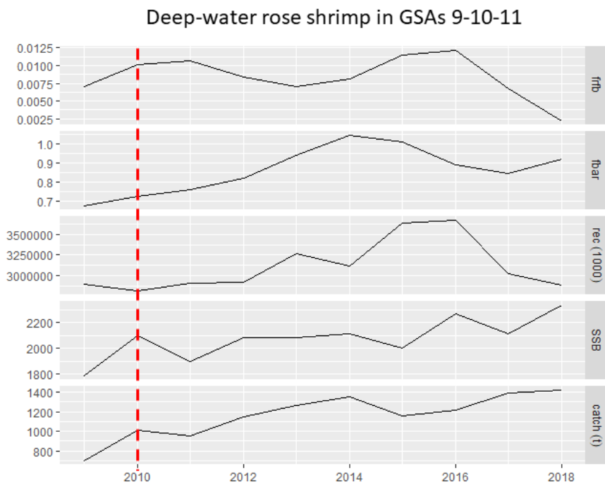
Figure 54. Deep-water rose shrimp in GSAs 9,10,11. Temporal development of the selectivity indicator ( frfb ) together with other key stock attributes. frfb : F of first
