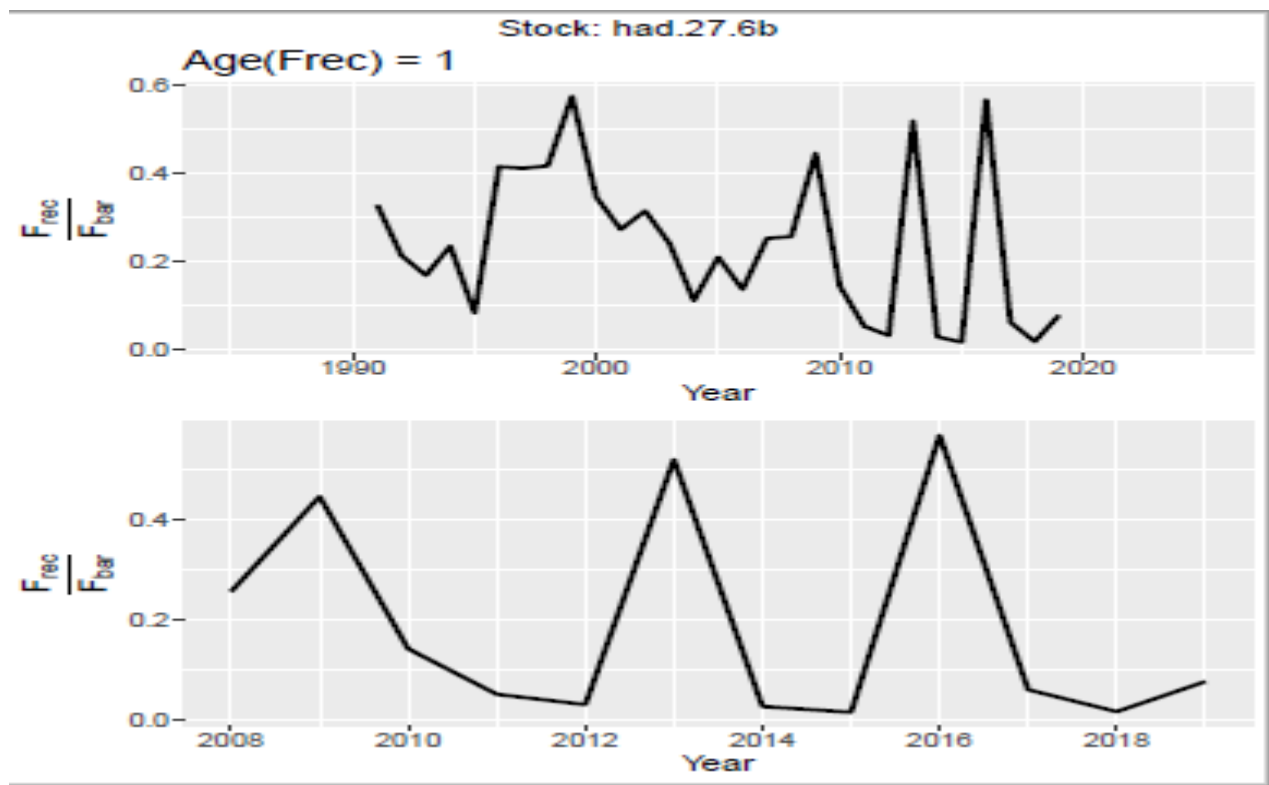
Figure 29: Haddock 27.6b. Time-series of Selectivity indicator F_{rec}/F_{bar} . Top: full time series; Bottom: reduced time series.
