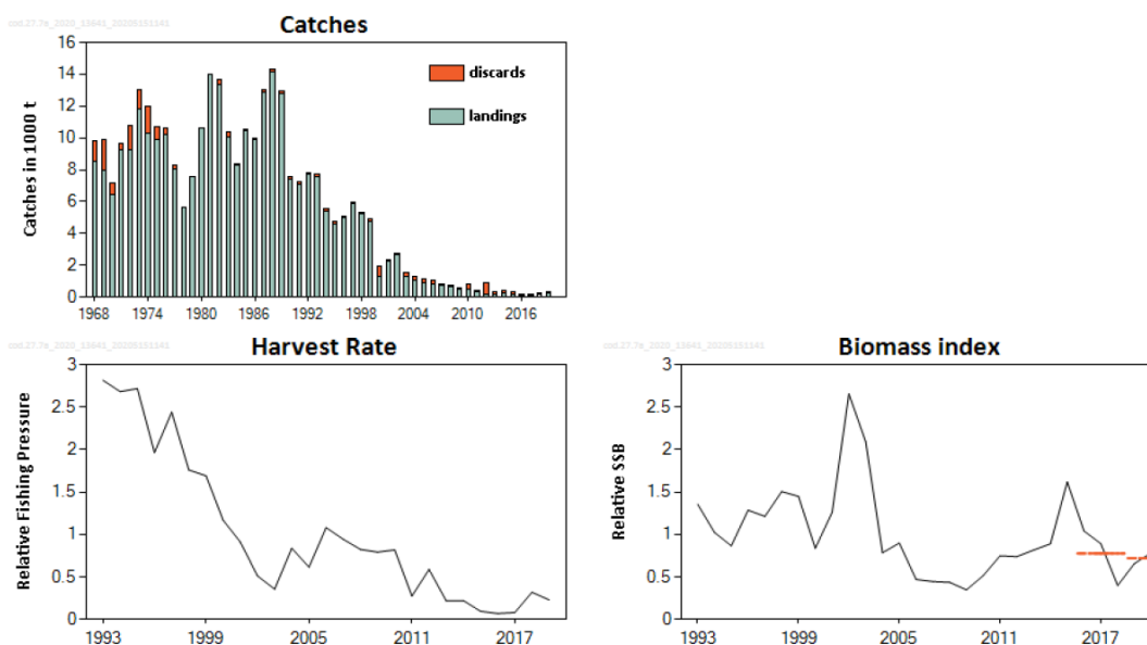
Figure 30: Irish Sea cod. Summary of the stock assessment. Figure taken from ICES 2020j.
