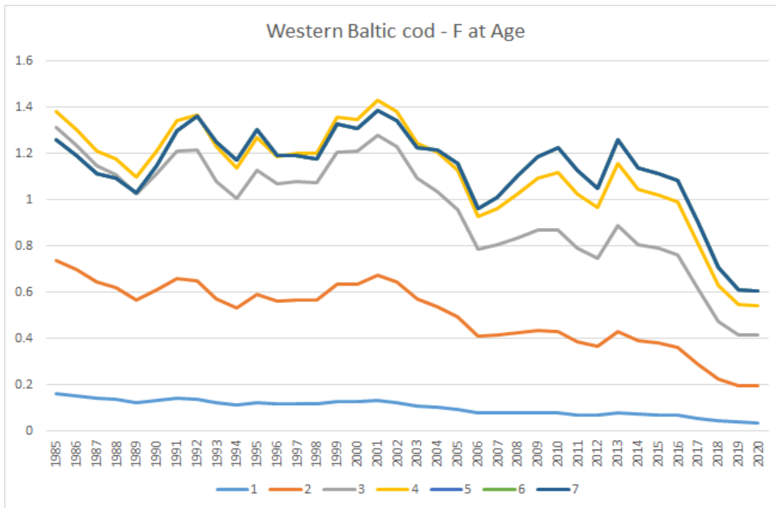
Figure 1: Example for time series of F at age-matrix as basis for calculated selectivity indicator F_{rec}/F_{bar} . F at age for the western Baltic Sea cod stock (ICES areas 22-24).
