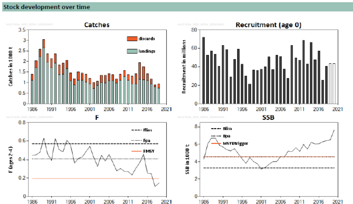
Figure 45: Four-spot megrim ( Lepidorhombus boscii ) in divisions 8.c and 9.a. Summary of the stock assessment. Figure taken from ICES 2019a
