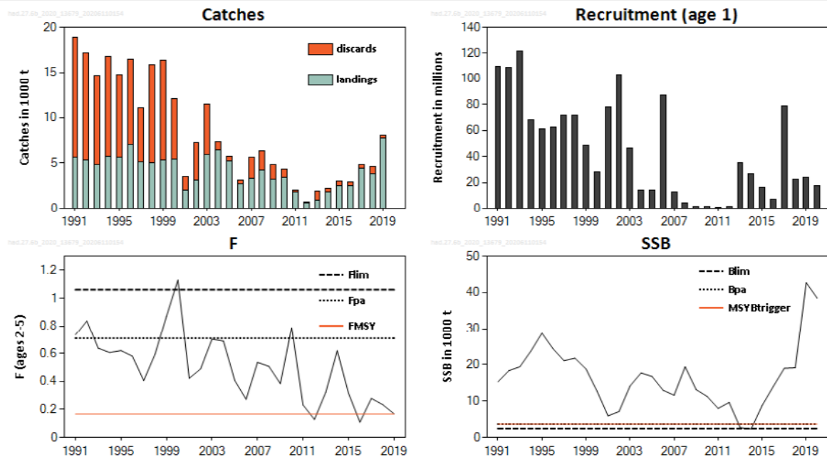
Figure 28: Rockall haddock. Summary of the stock assessment. Figure taken from ICES 2020c.
