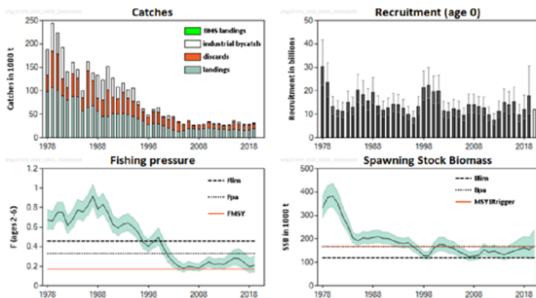
Figure 16: North Sea whiting. Summary of the stock assessment. Recruitment, F and SSB show confidence intervals (95%) in the plot. Figure taken from ICES 2020e.
